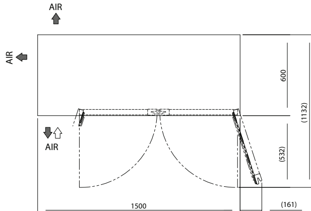
VIEW A(1/10)
